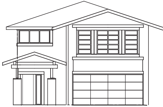
1102 Cawthra Court, Coquitlam - south elevation
